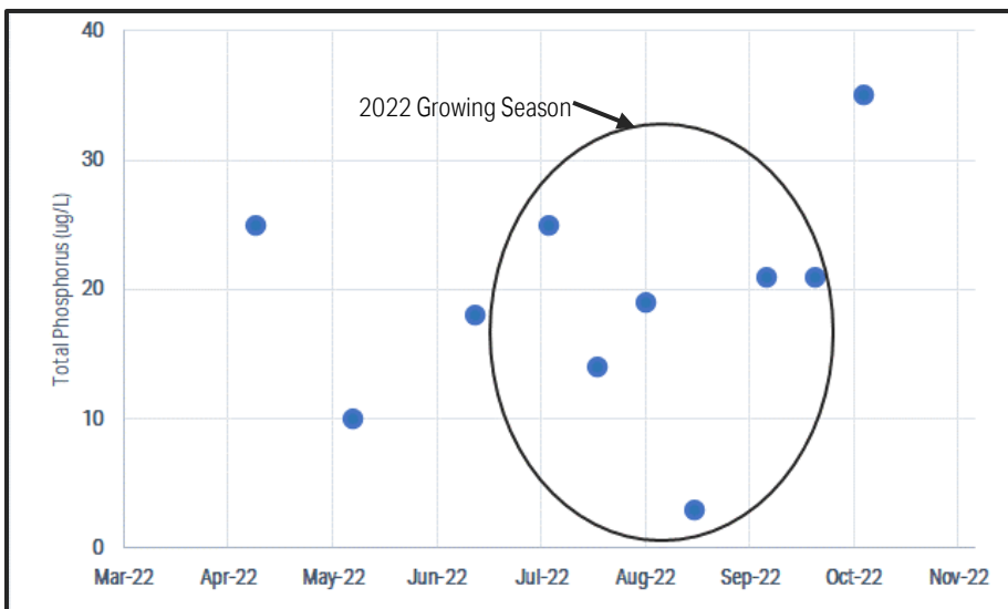
Figure 5. Monthly Total Phosphorus Concentrations, Chatfield Reservoir, 2022.
