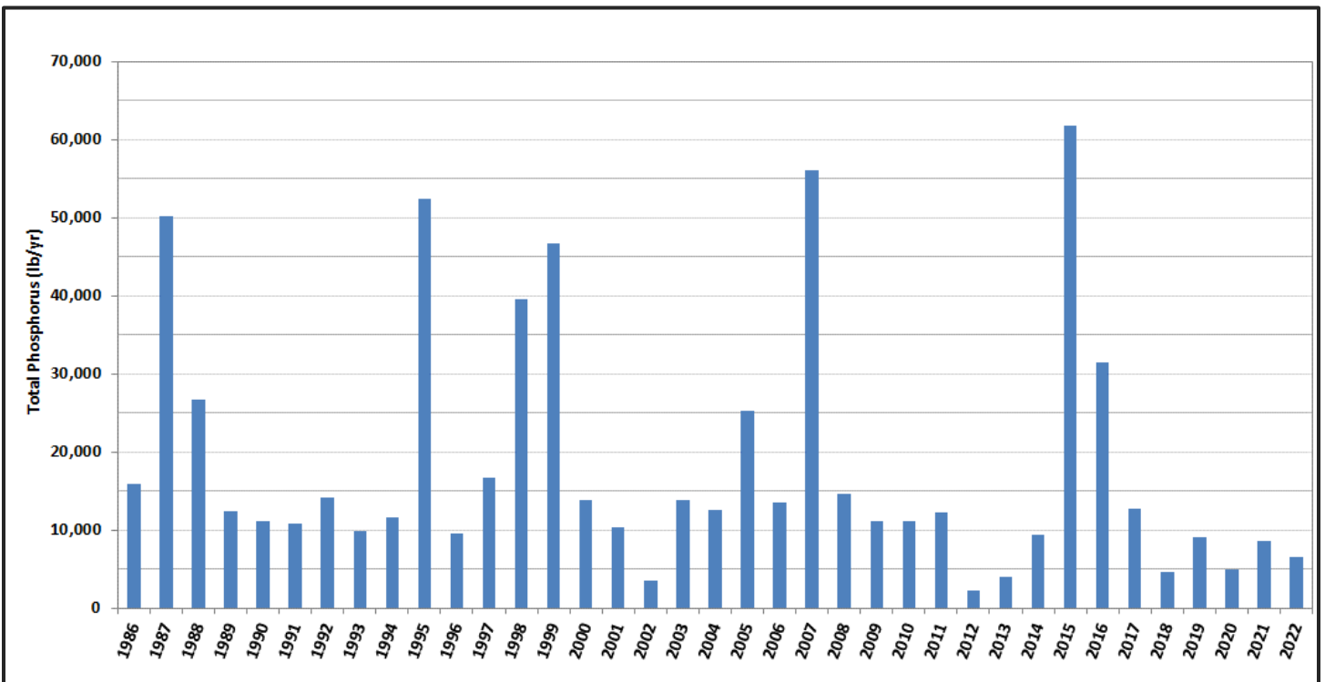
Figure 7. Calculated Annual TP Loads to Chatfield Reservoir from 1986 to 2022
