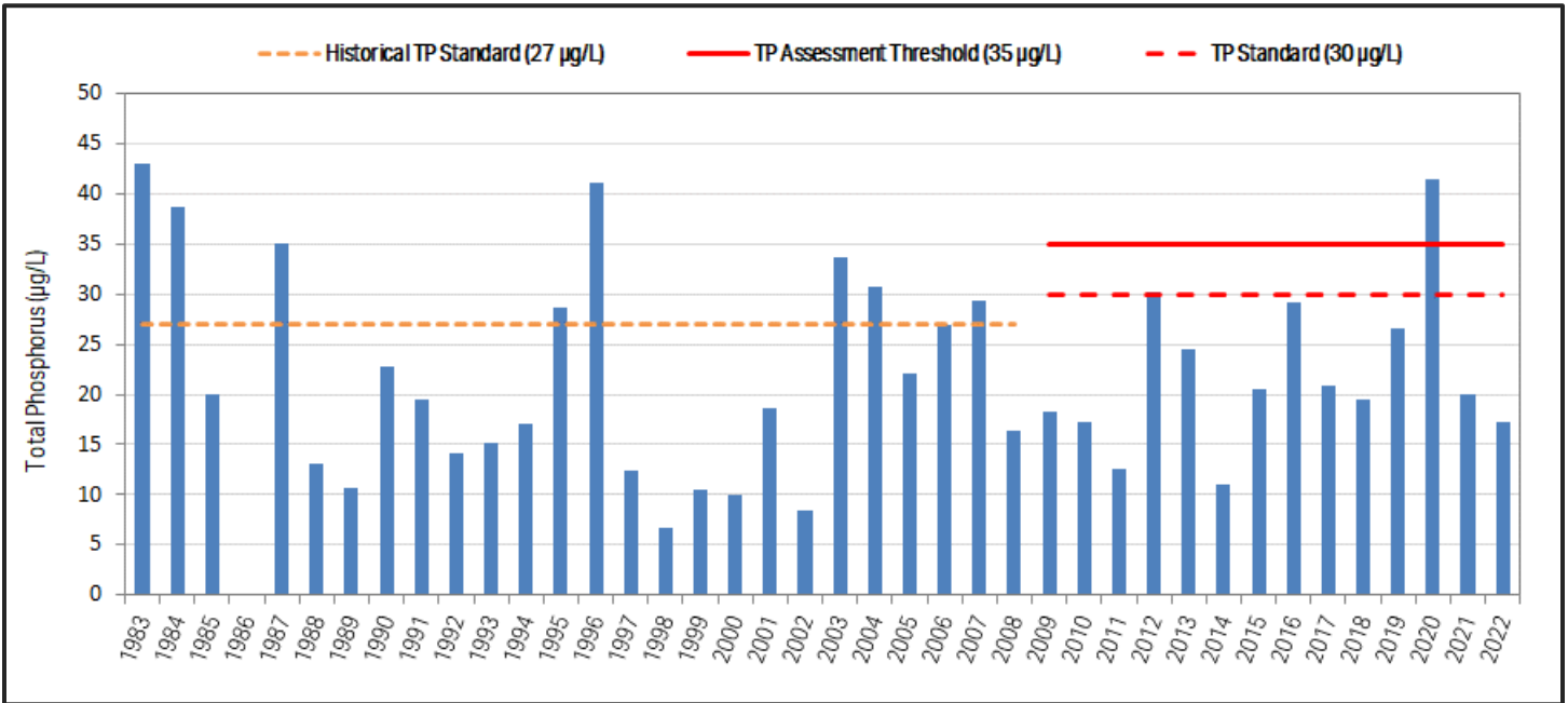
Figure 4. Growing Season Average Total Phosphorus Concentrations, Chatfield Reservoir, 1983-2022.
