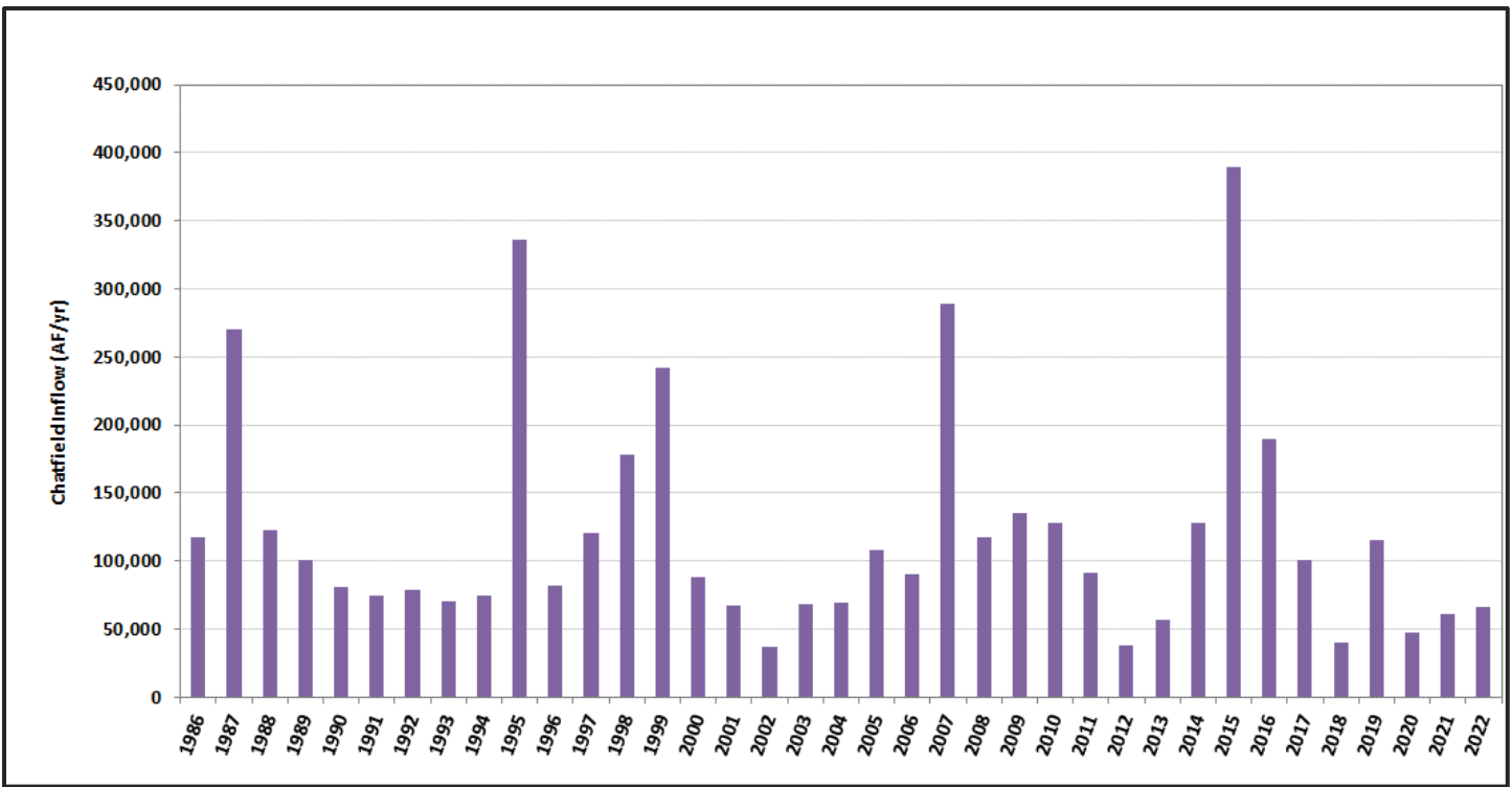
Figure 8. Chatfield Reservoir Calculated Annual Inflow (1986–2022)
