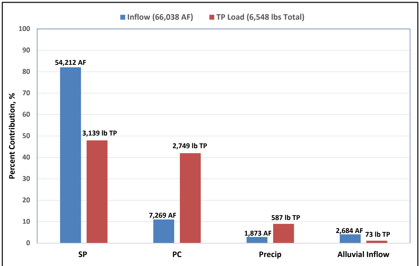
Figure 9. 2022 Chatfield Reservoir Inflows and TP Loads by Source.
